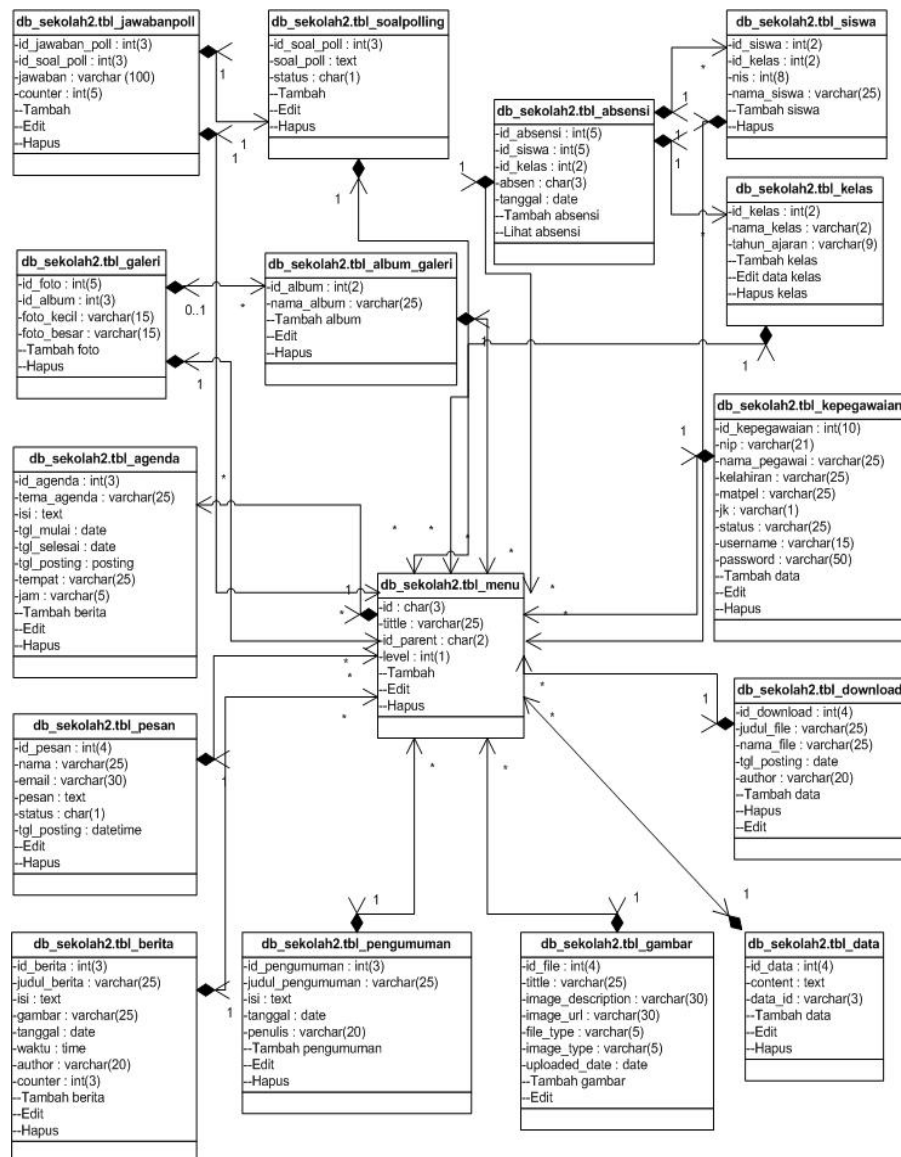
Gambar 3.4 Class Diagram
